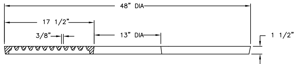
GRATE SECTION
